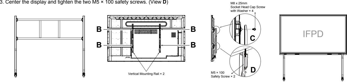
Front View of Fully Assembled Mobile Stand
